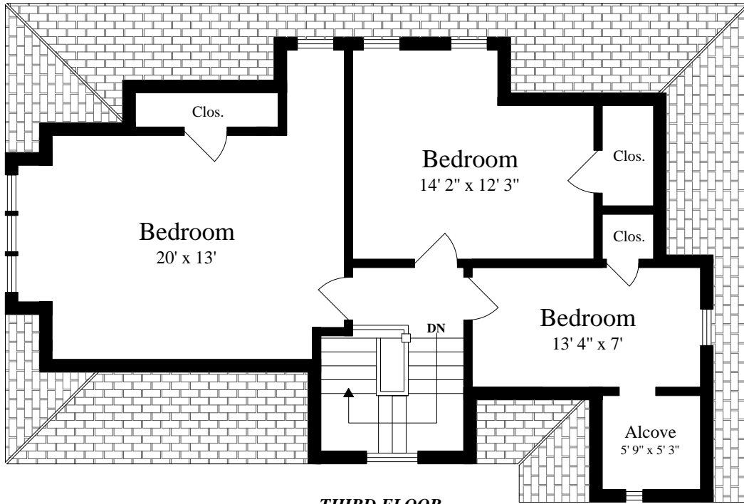
THIRD FLOOR Apartment #2
