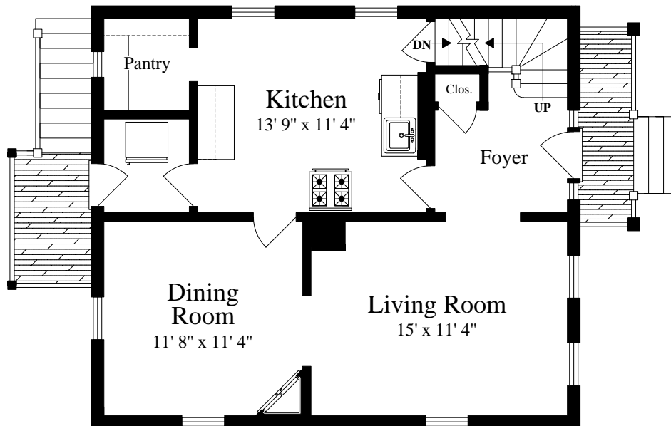
FIRST FLOOR
