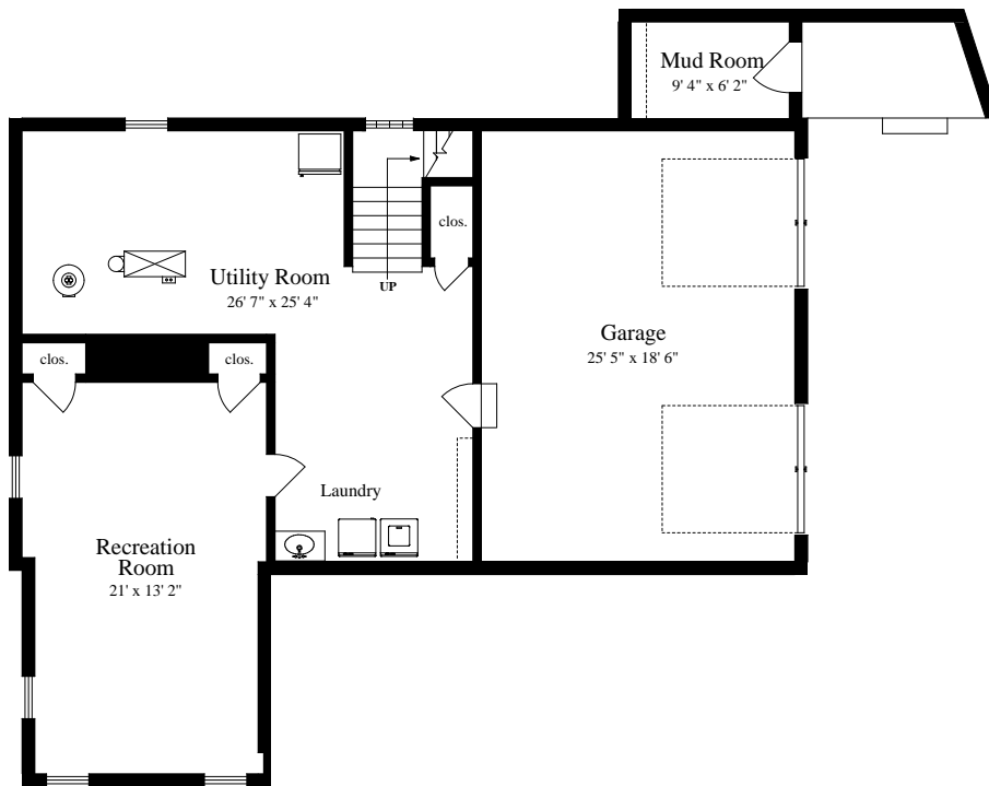
LOWER LEVEL
